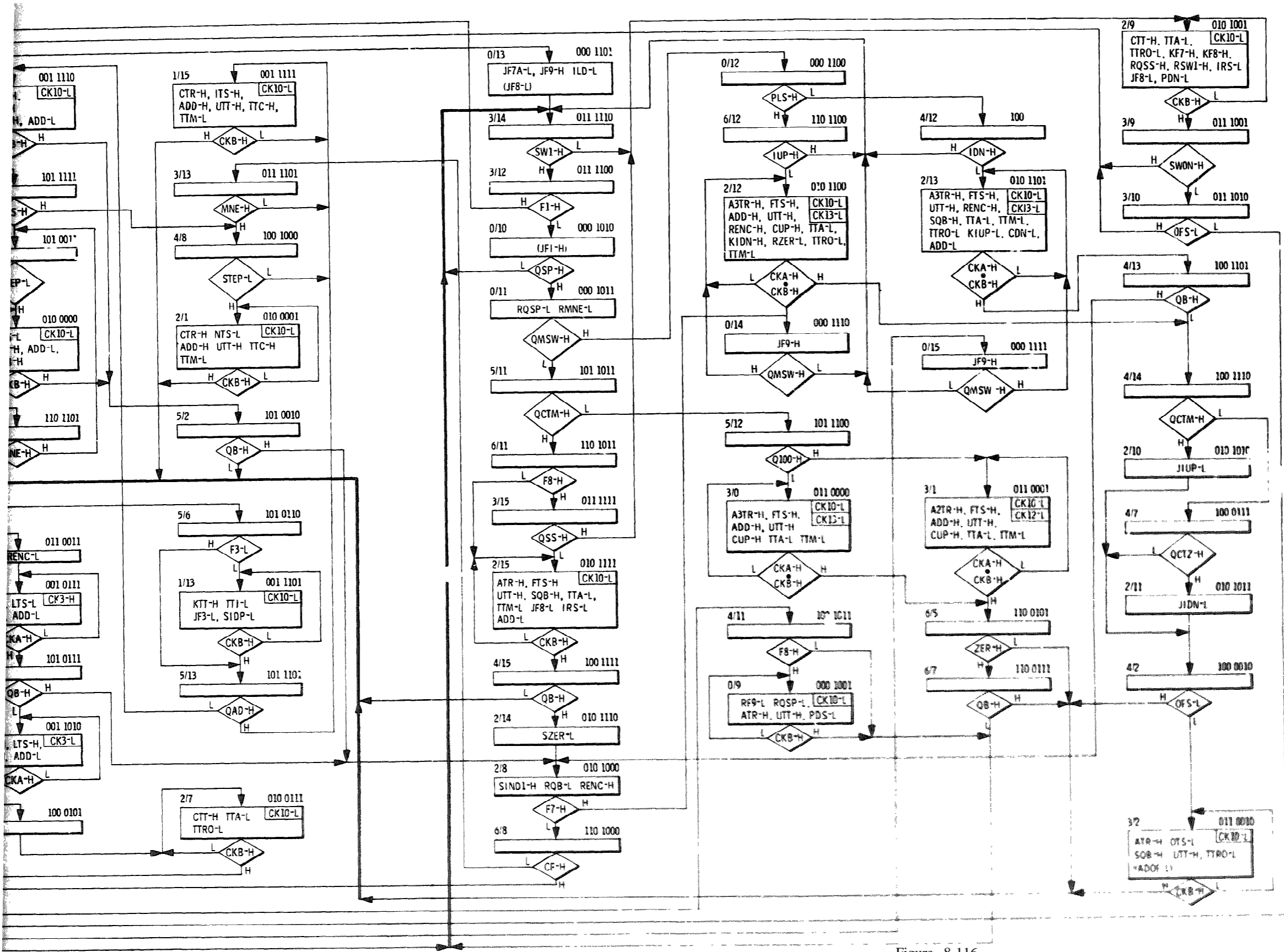
Figure 8-116. DCU Algorithmic State Machine (Flow Graph) 8-155
