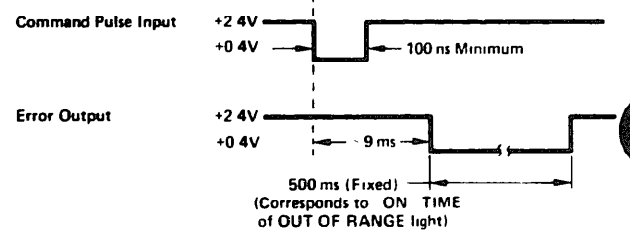
Figure 3-2. Model 8660B Timing
