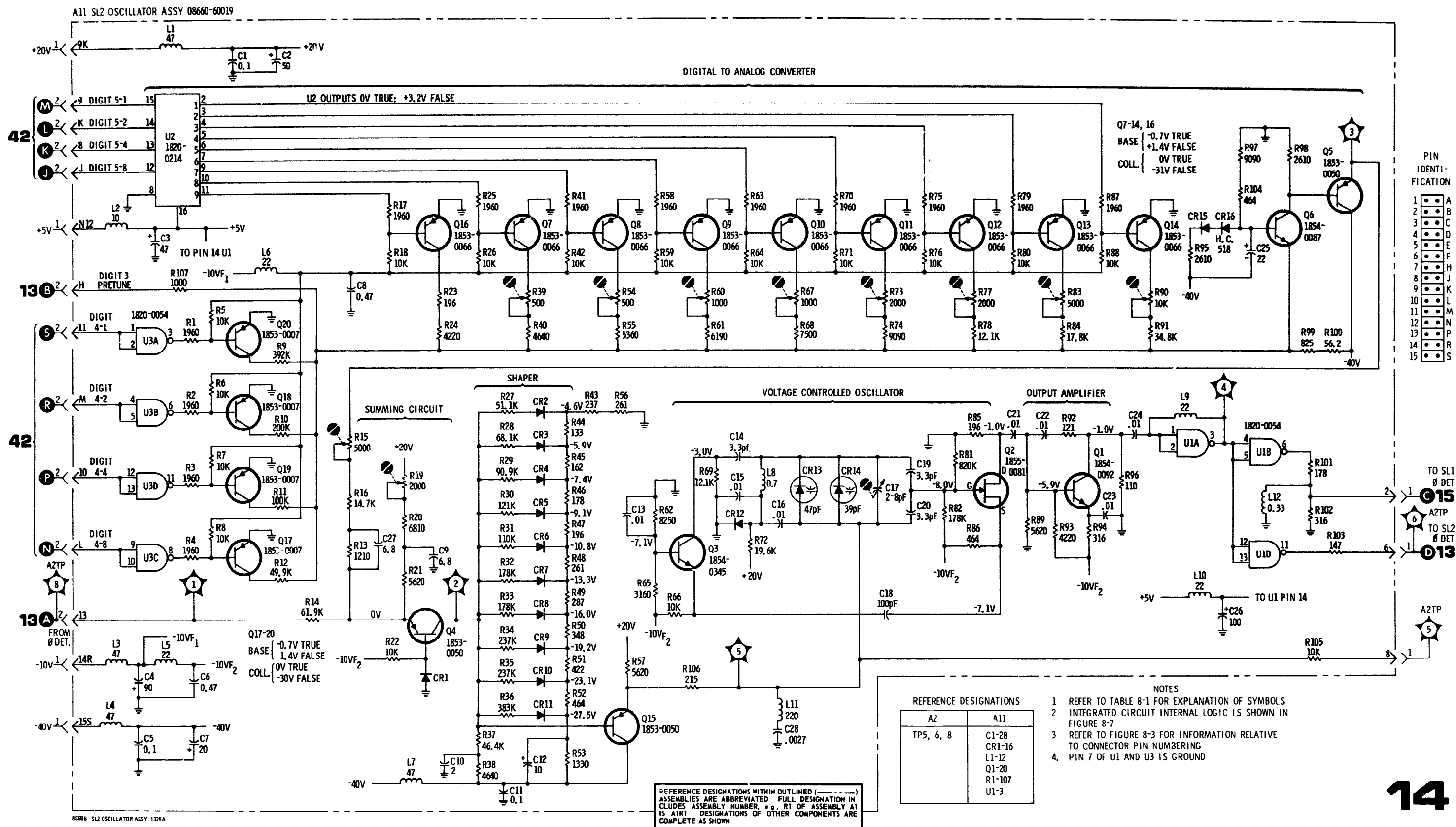
Figure 8-45. SL2 VCO Schematic
