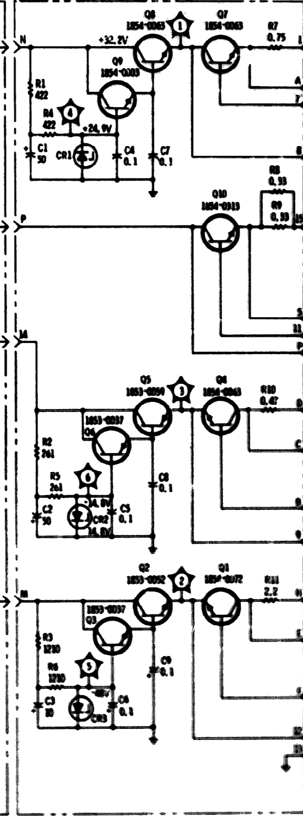
A6A1 PREREGULATOR ASSY 08660-60024
