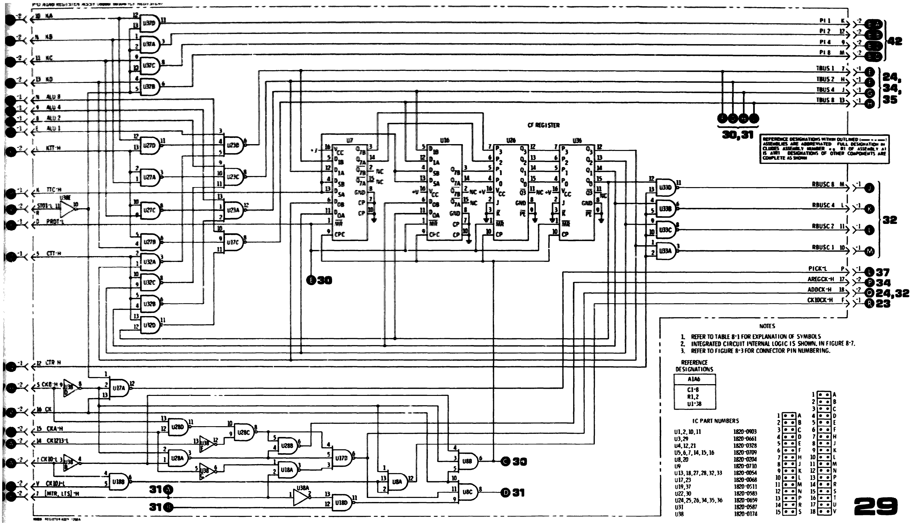
Figure 8-77. P/O AIA6 Register Assy (Part 1)
