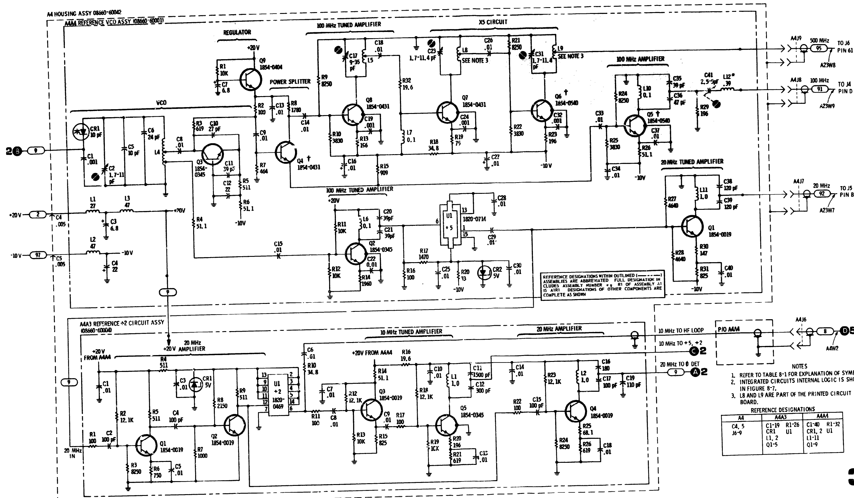
Figure 8-19. Reference VCO and Divider Schematics
