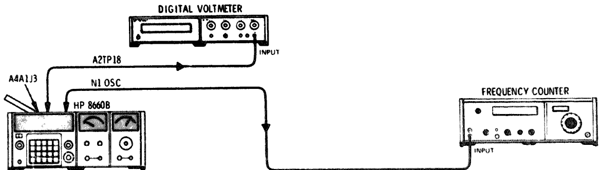
Figure 5-12. N1 Loop Test Setup
