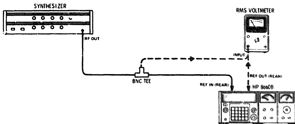
Figure 4-3. Reference Output Test Setup
