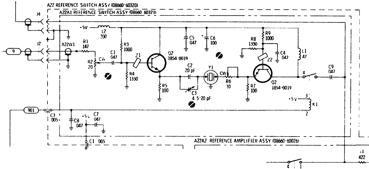
Figure 8-16. Reference Circuit Schematics (Partial Diagram, Part of Change 6)
