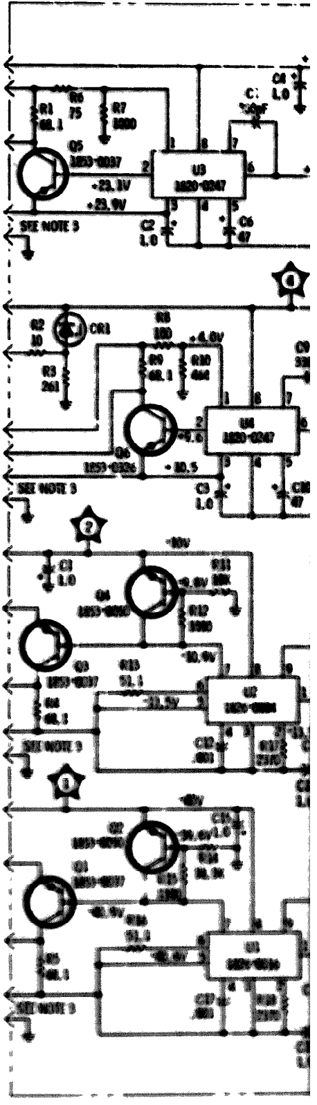
A5 REGULATOR ASSY 08660-60023
